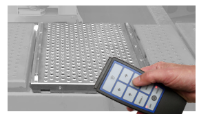
Play detector with remote control for the 4.65 S
