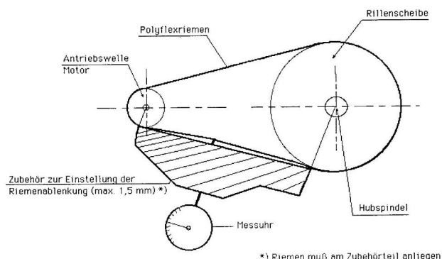
Figure 16: Measurement instrument
