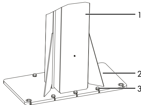
Figure 22: Anchoring
