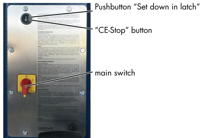
Figure 4: Operating unit
